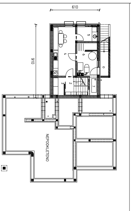
DELNA KLET M=1:200
